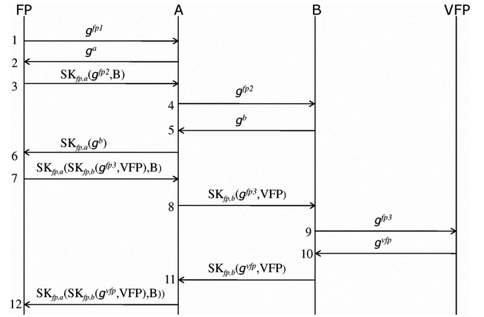
Fig. 2. Anonymous channel establishment
