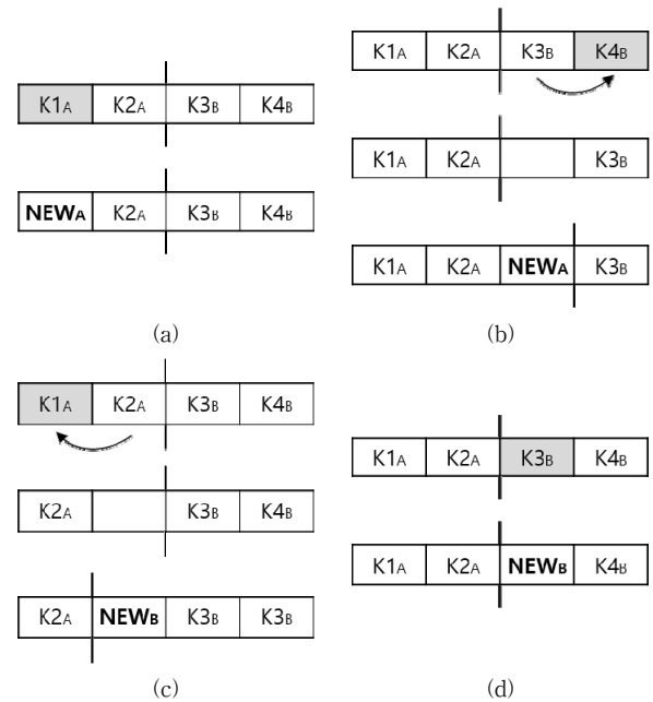
Fig. 4. Example of the Insertion Process when Kick-out Process is Needed
