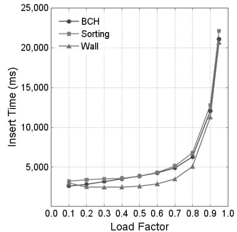
Fig. 10. Comparison of Insert Time
