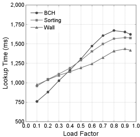
Fig. 8. Comparison of Negative Lookup Time
