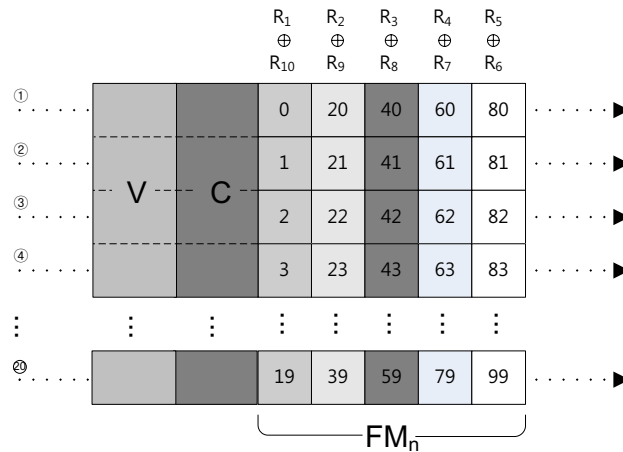
Fig. 3. MIXED_MEM(using SHA-1)
