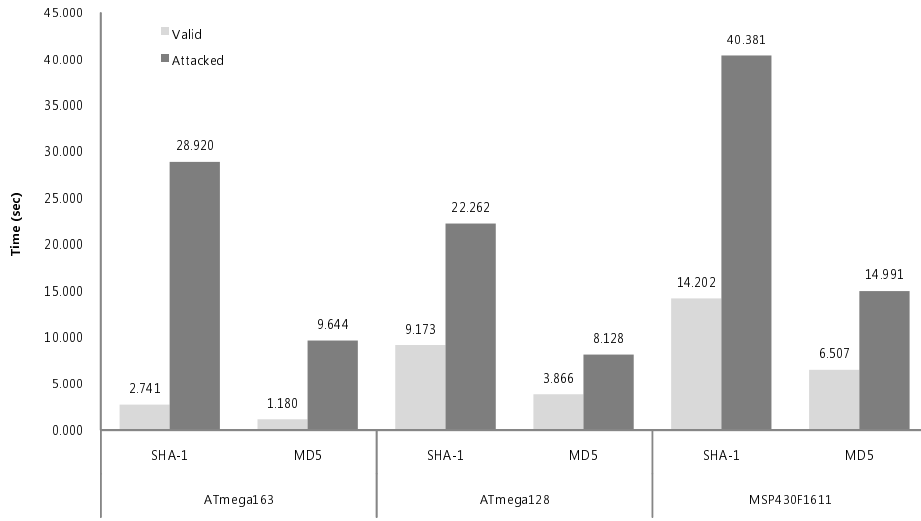
Fig. 5. The comparison between total verification time of valid nodes and malicious nodes. The time of malicious nodes at least doubles that of valid nodes.
