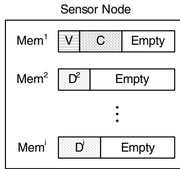
Fig. 1. Memory contents in a sensor node. Mem^1 is a RAM of micro controller and Mem^i (i > 1) is programmable flash memory.
